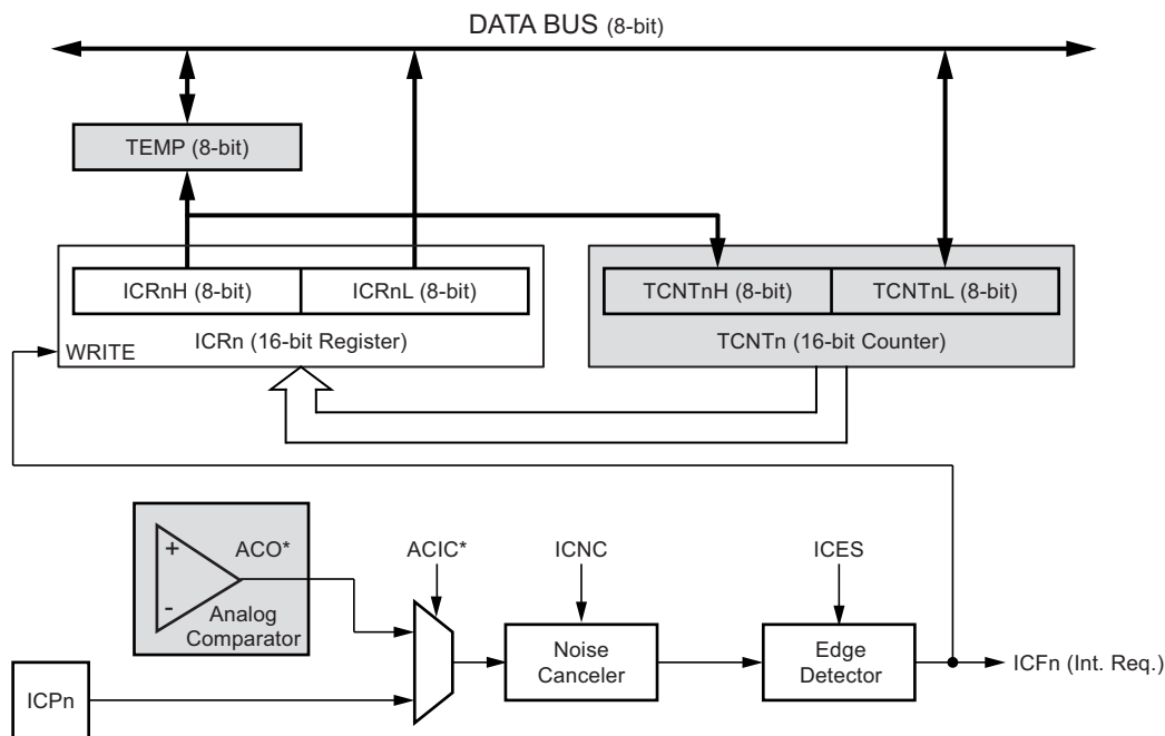
Figure 21-3. Input Capture Unit Block Diagram
